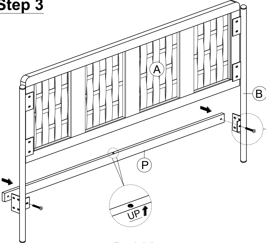
Back View
